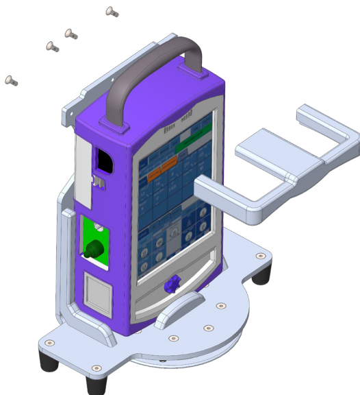
EnVe/ReVel Bracket Installation
