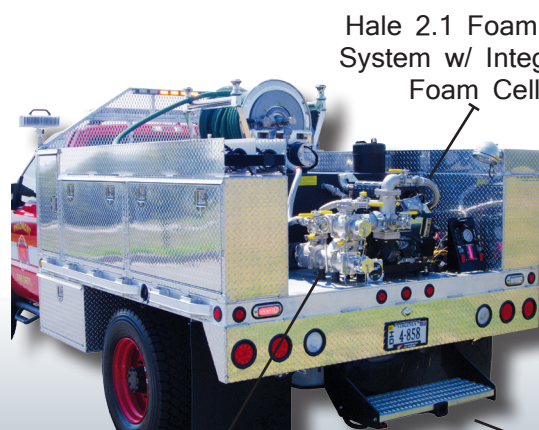
Hale All Stainless Pump & Stainless Plumbing
