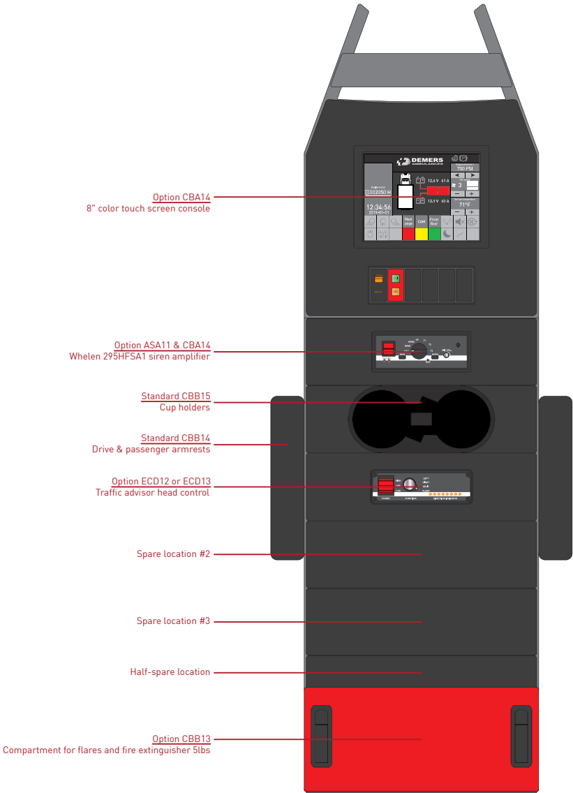
Top view
