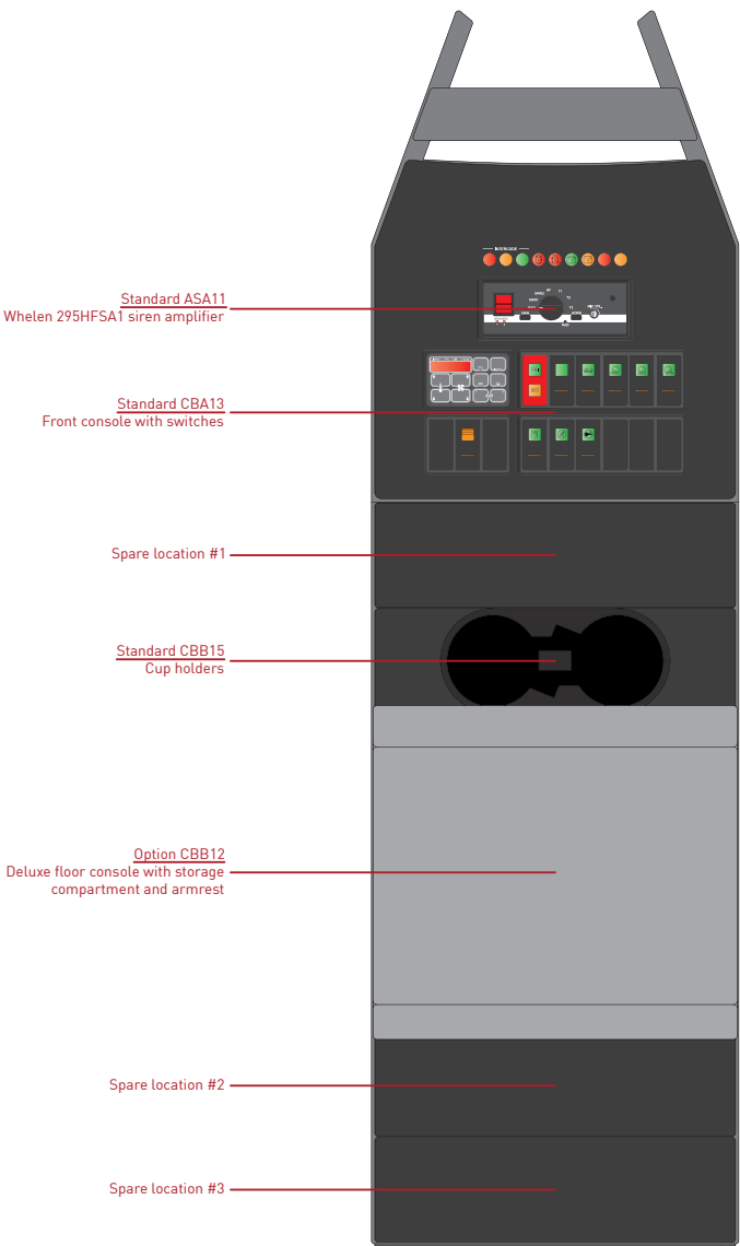
Top view
