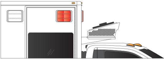
Custom Option CVC-AUX-12 60000 BTU auxiliary dual in-line condenser installed on front of module. Hoseline, model TMC2014
