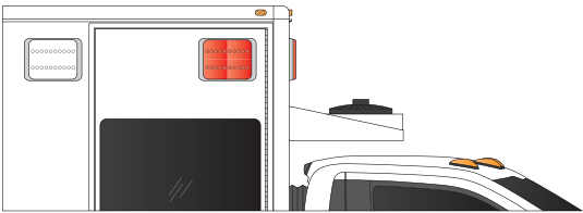
Custom Option CVC-AUX-11 45000 BTU auxiliary dual in-line condenser installed on front of module. Hoseline, model TMC2007
